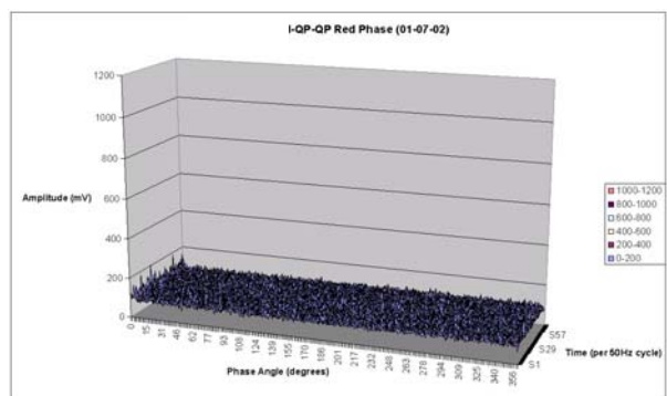
Figure 4b: PD Activity after joint replacement
