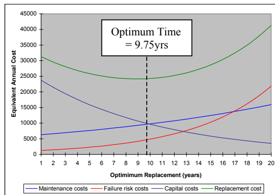
Figure 5: An Asset Management DSS for MV Plant
