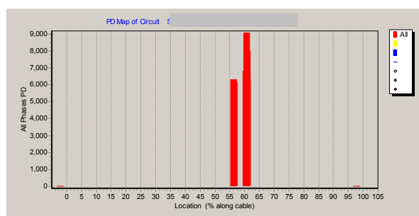
Figure 3 : On-Line PD Map of 33kV 'Mixed' Cable
