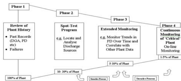
FIGURE 2: 4-PHASE APPROACH FOR CONDITION ASSESSMENT OF MV PLANT
