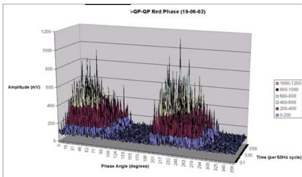
Figure 4a : PD Activity before joint replacement
