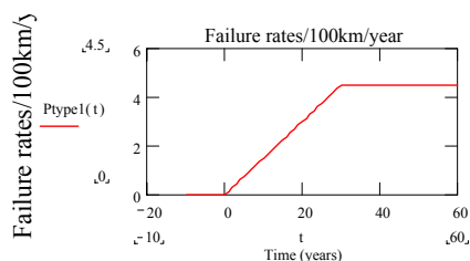
Figure 6: MIPC Failure Rates with Age in Service
