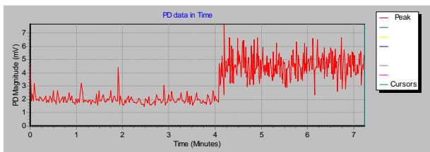
Fig 4 PD recording with and without noise reduction
