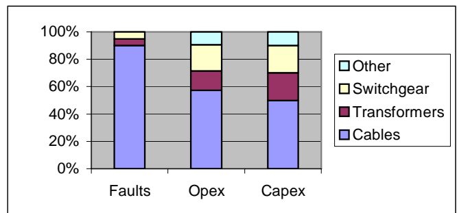
Fig 2 Contributions to faults, operational, & capital expenditure from different plant types
