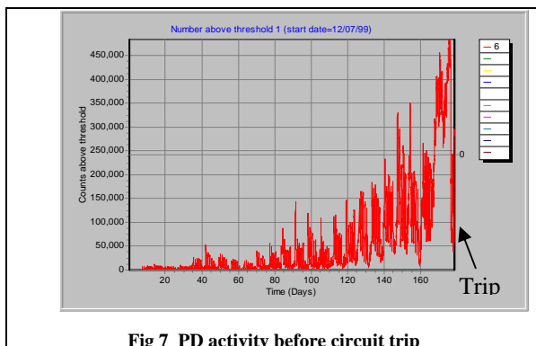
Fig 7 PD activity before circuit trip
