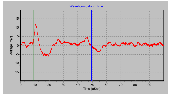
Fig 5 On-line PD mapping waveform
