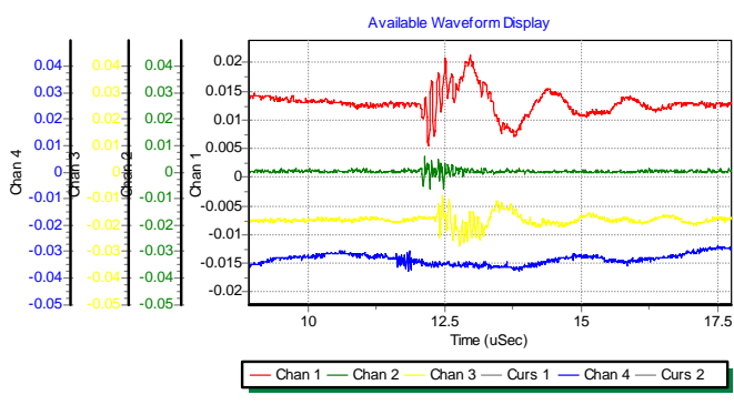
Fig 3 Noise on various sensors on switchgear
