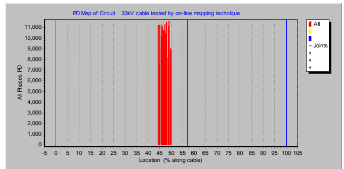
Fig 6 On-line PD map of 33kV cable
