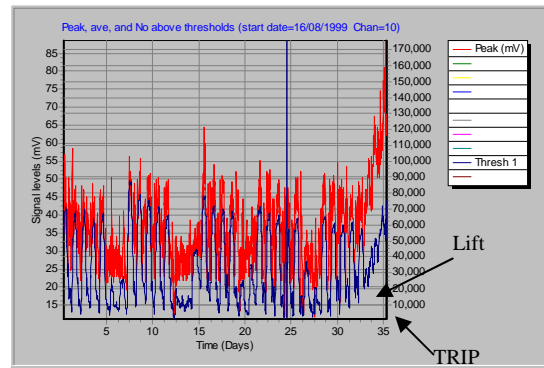
Fig 8 PD behaviour prior to failure
