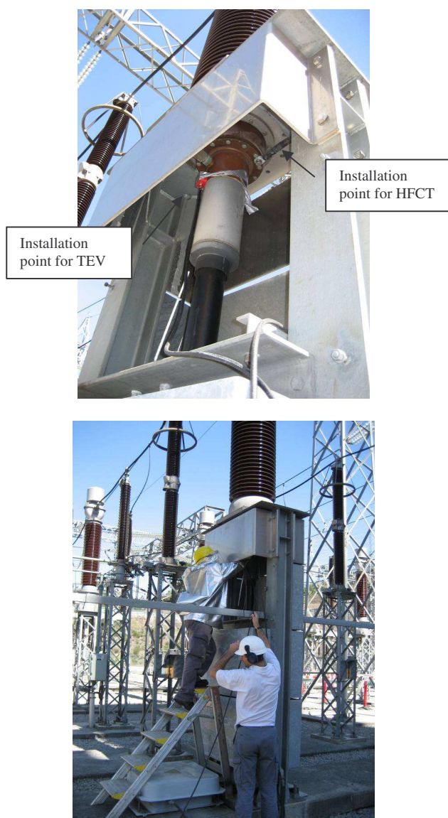
Figure 17: TEV & HFCT Sensor connection and attachment at base of 220kV cable sealing end
