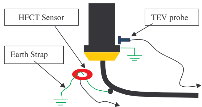
Figure 16: Sensor Connection for HV Cable Testing
