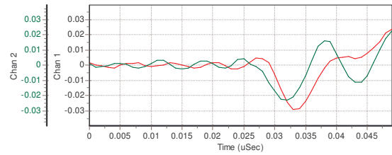
Figure 12: Time Of Flight Measurement for PD Site Location using 2x TEV sensors on an AIS panel
