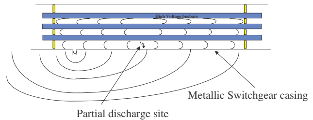
Figure 8: Transient earth voltage radiation of PD
