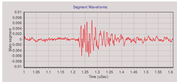
Figure 10: Switchgear PD pulse in 11kV metal clad AIS
