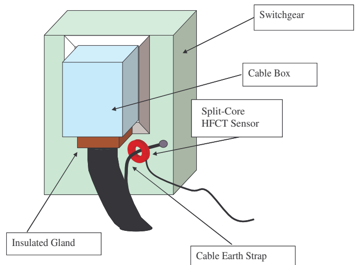
Figure 1: HFCT Sensor Connection on Cable Earth Strap for On-Line PD Testing
