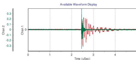
Figure 14: 25kV VT PD pulse detected by TEV sensor (green) and HFCT (red) on
