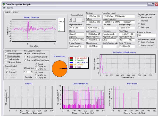
Figure 11 PDGold© Switchgear PD Event Recogniser Page
