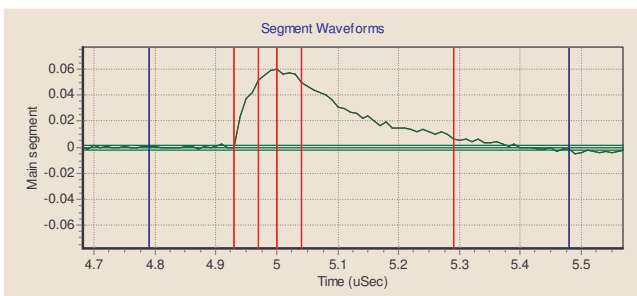
Figure 3: Pulse from a PD site in a cable
