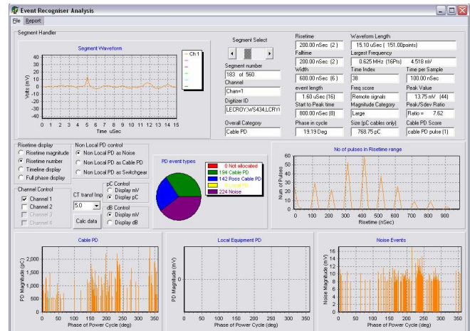
Figure 4: PDGold© Software Event Recogniser Page
