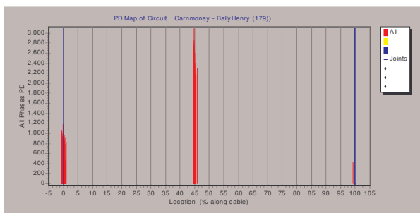
Figure 7: PD Map of ‘mixed’ 33kV PILC/XLPE Cable
