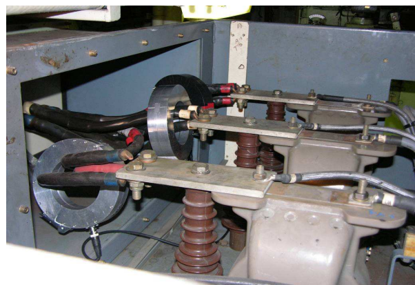
Figure 15: HFCT Connections on 6.6kV Generator
