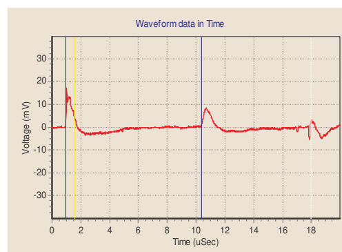
Figure 5: ‘Single-Ended’ PD location method
