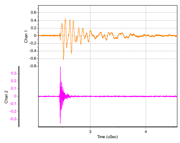
Figure 5: 25kV VT Internal PD pulse Shape
