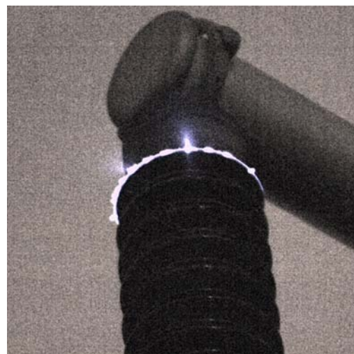
Figure 1: Low-light Photo of Surface Discharge
