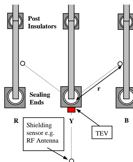
Figure 4: Sensor Positions for Shielded Measurement
