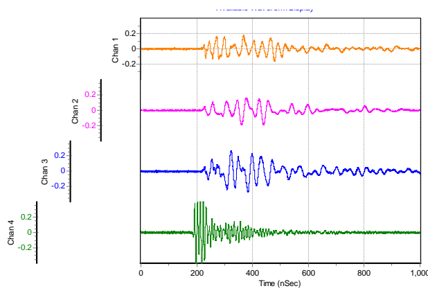
Figure 3: Corona discharge pulse waveforms
